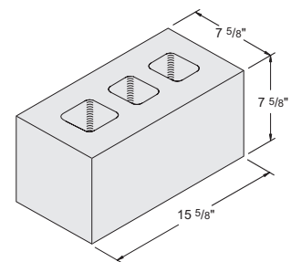
8" x 8" x 16" 75% Solid #1030410
