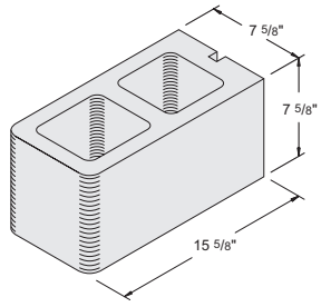
8" x 8" x 16" Bullnose Double-End #1030260
