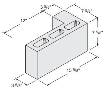
4" x 8" x 16" L Corner #1050160
