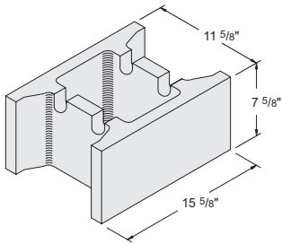
12" x 8" x 16" Grout #1010220
