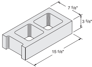
8" x 4" x 16" Half High #1030180
