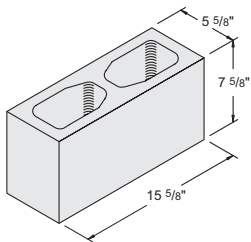
6" x 8" x 16" Hollow Stretcher #1040000
