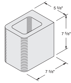
6" x 8" x 8" Half Bullnose Double-End #1040250
