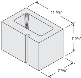
12" x 8" x 8" Half #1010030
