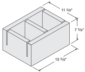
12" x 8" x 16" Bond Beam Knock-Out #1010050
