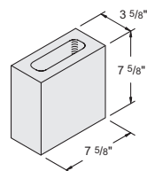
4" x 8" x 8" Half #1050190
