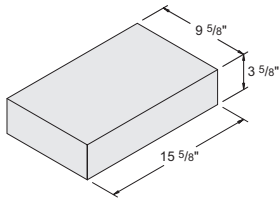
10" x 4" x 16" Solid #1050090
