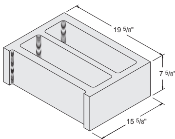
20" x 8" x 16" Hollow Stretcher #1061520
