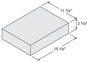
12" x 4" x 16" Solid #1050100
