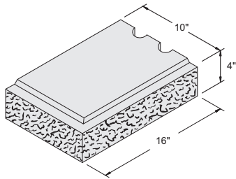
16" x 4" x 10" Dual Lock Left End #1061081
