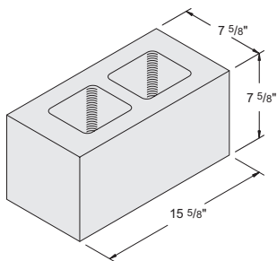
8" x 8" x 16" 57% Solid #1030340
