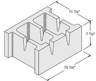
12" x 8" x 16" Drain #1010012
