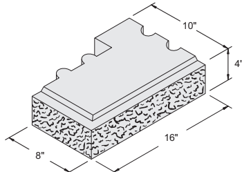
16" x 4" x 10" x 8" Dual Lock Left Corner #1061071
