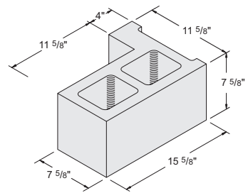
12" x 8" x 16" L Corner #1010010
