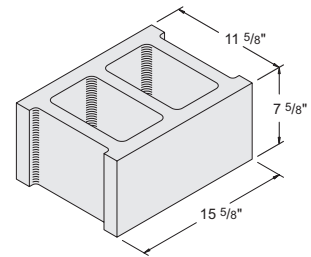
12" x 8" x 16" Hollow Stretcher #1010000
