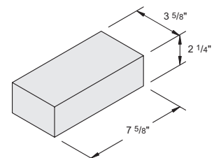
4" x 2 1/4" x 8" Concrete Brick #1062000
