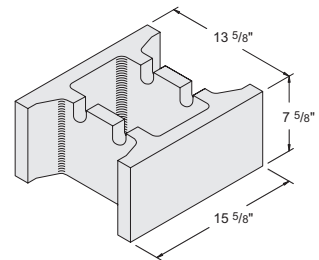
14" x 8" x 16" Grout #1060010
