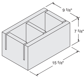
10" x 8" x 16" Bond Beam Knock-Out #1020100
