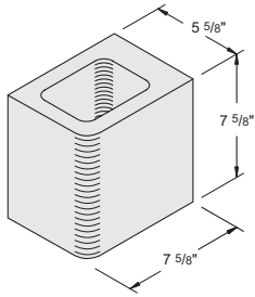
6" x 8" x 8" Half Bullnose Single-Face #1040240
