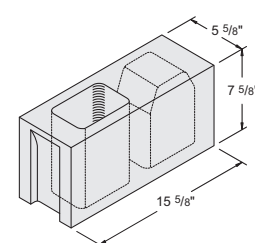
6" x 8" x 16" Anchor Bolt #1040002
