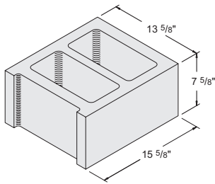
14" x 8" x 16" Hollow Stretcher #1060000
