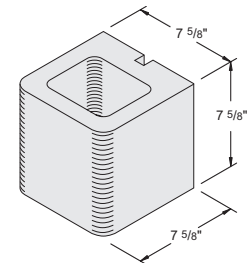
8" x 8" x 8" Half Bullnose Double-End #1030290
