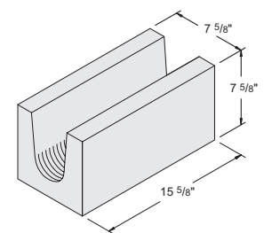
8" x 8" x 16" U-Shaped Lintel #1030110
