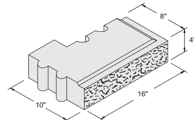
16" x 4" x 10" x 8" Dual Lock Right Corner #1061072
