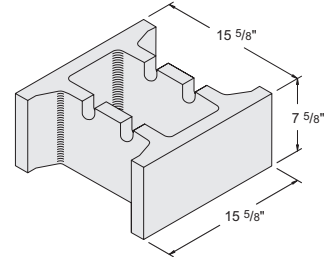
16" x 8" x 16" Grout #1061030
