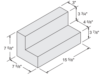
8" x 8" x 16" 4x4 Cut Out Solid Header #1030175
