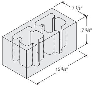
8" x 8" x 16" Soundblox® RSC RF #1030330
