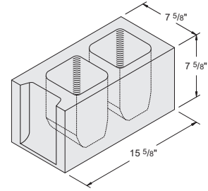
8" x 8" x 16" Termite #1030040
