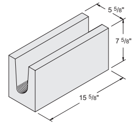
6" x 8" x 16" U-Shaped Lintel #1040260
