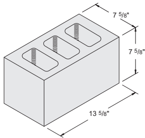
8" x 8" x 14" #1030270 ALT: 14" Half
