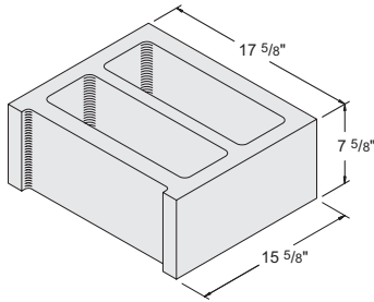
18" x 8" x 16" Hollow Stretcher #1061500
