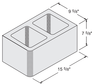
10" x 8" x 16" Bullnose Single-Face #1020130
