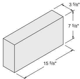
4" x 8" x 16" Solid #1050080
