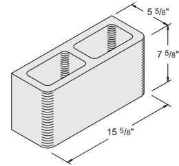
6" x 8" x 16" Bullnose Double-Face #1040070
