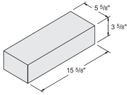
6" x 4" x 16" Solid #1050070
