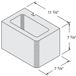
12" x 8" x 8" Half Bullnose Single-Face #1010590
