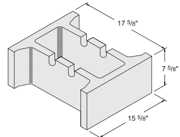
18" x 8" x 16" Grout #1061510
