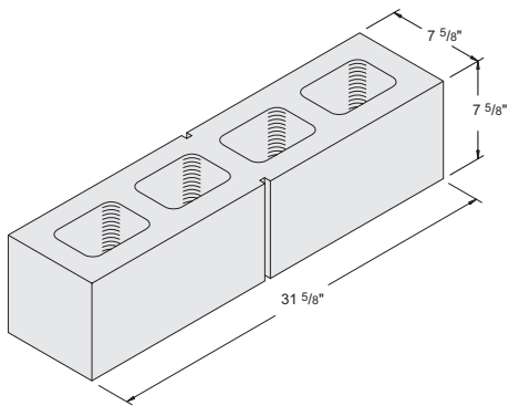
8" x 8" x 32" Double 8 Regular - #1030950 Light Weight - #1030940
