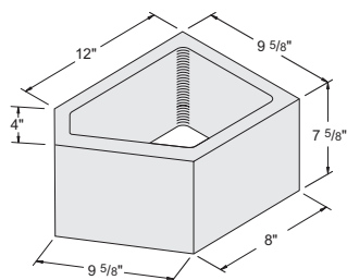
10" 45° Angle #10200020
