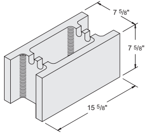
8" x 8" x 16" Grout #1030230
