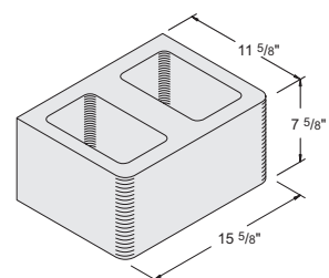
12" x 8" x 16" Bullnose Double-Face #1010550
