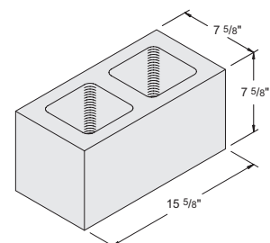
8" x 8" x 16" Pier #1030050
