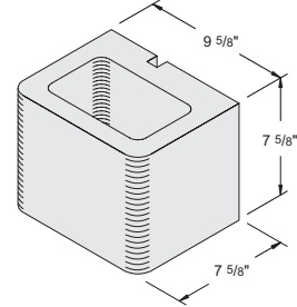
10" x 8" x 8" Half Bullnose Double-End #1020180
