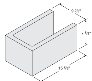
10" x 8" x 16" Beam Lintel (Hairpin) #1020280
