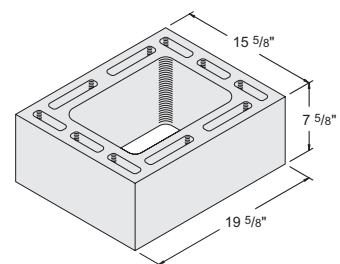
8" x 12" Chimney Block #1088772
