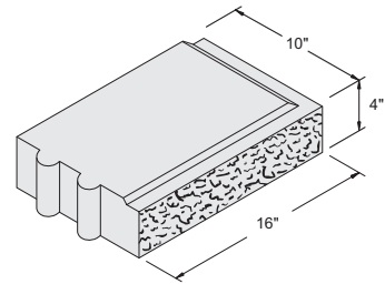
16" x 4" x 10" Dual Lock Right End #1061082
