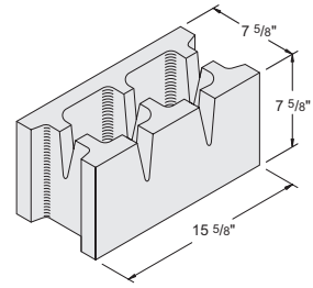
8" x 8" x 16" Drain #1030002
