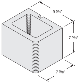
10" x 8" x 8" Half Bullnose Single-Face #1020170
