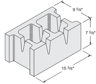
10" x 8" x 16" Drain #1020080
