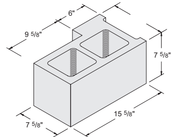
10" x 8" x 16" L Corner #1020010
