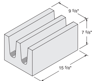
10" x 8" x 16" U-Shaped Lintel #1020260
