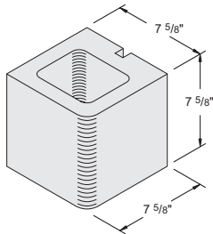
8" x 8" x 8" Half Bullnose Single-Face #1030280
