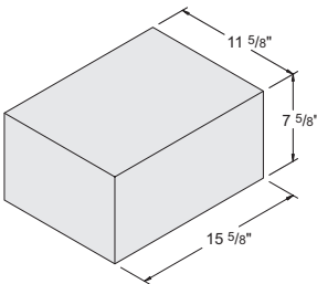
12" x 8" x 16" Solid #1010160
