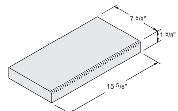
8" x 2" x 16" Curb #1063025
