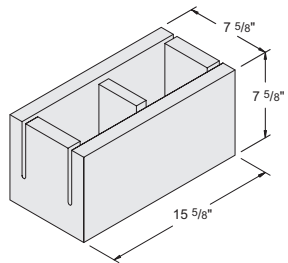
8" x 8" x 16" Bond Beam Knock-Out #1030120
