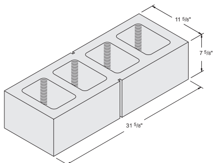
12" x 8" x 32" Double 12 Regular - #1010920 Light Weight - #1010930
