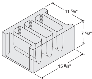
12" x 8" x 16" Termite #1010040
