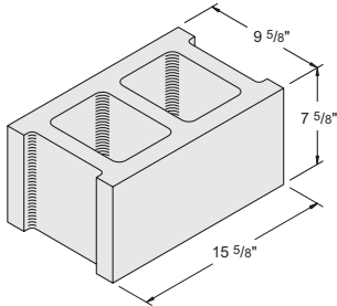
10" x 8" x 16" Hollow Stretcher #1020000
