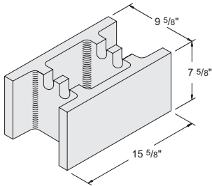
10" x 8" x 16" Grout #1020070
