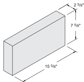
3" x 8" x 16" Solid #1063010
