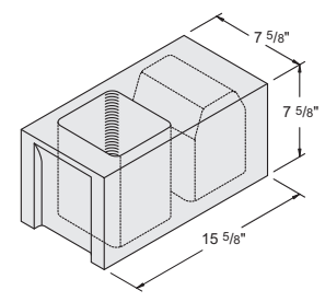
8" x 8" x 16" Anchor Bolt #1030041
