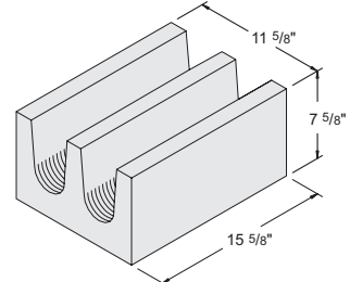
12" x 8" x 16" U-Shaped Lintel #1010200
