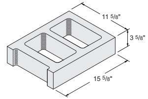
12" x 4" x 16" Half High #1010180 MIXED: Jamb 1:1 Ratio
