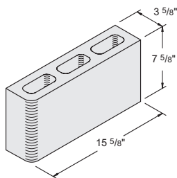
4" x 8" x 16" Bullnose Single-Face #1050400
