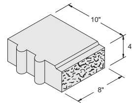
8" x 4" x 10" Dual Lock Right Half #1061062
