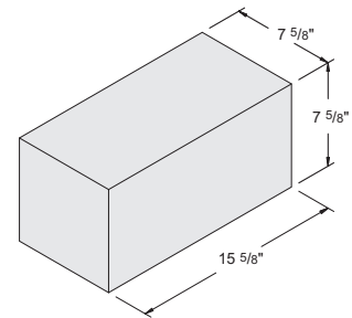
8" x 8" x 16" Solid #1030140
