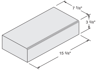
8" x 4" x 16" Curb #1050085
