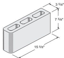
4" x 8" x 16" Bullnose Double-End #1050410
