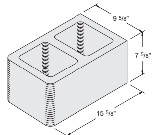
10" x 8" x 16" Bullnose Double-End #1020190
