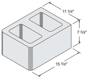
12" x 8" x 16" Bullnose Double-End #1010540
