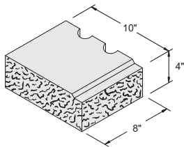
8" x 4" x 10" Dual Lock Left Half #1061061
