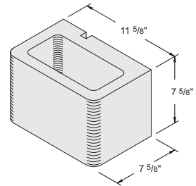
12" x 8" x 8" Half Bullnose Double-End #1010600
