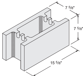
8" x 8" x 16" Grout Item #1030230 108 units / pallet • 35 lbs. / unit
