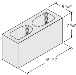
6" x 8" x 16" Hollow Stretcher Item #1040000 132 units / pallet • 29.3 lbs. / unit
