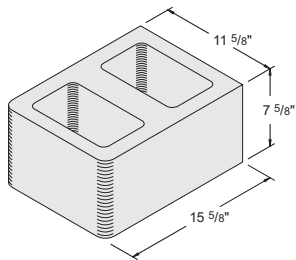
12'' x 8'' x 16'' Bullnose Double-End Item #1010540 78 units / pallet • 50 lbs. / unit
