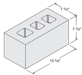
8'' x 8'' x 16'' 75% Solid Item #1030410 54 units / pallet • 68.5 lbs. / unit
