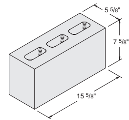
6" x 8" x 16" 75% Solid Item #1040200 96 units / pallet • 44 lbs. / unit
