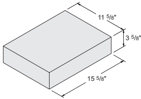
12'' x 4'' x 16'' Solid Item #1050100 72 units / pallet • 54 lbs. / unit
