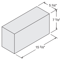
6" x 8" x 16" Solid Item #1040020 72 units / pallet • 50 lbs. / unit
