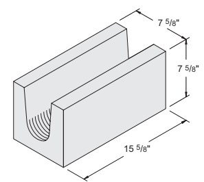
8" x 8" x 16" U-Shaped Lintel Item #1030110 108 units / pallet • 42.7 lbs. / unit
