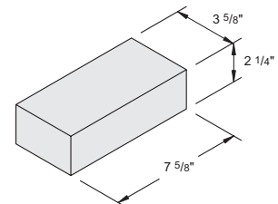
4'' x 2 1/4'' x 8'' Concrete Brick Item #1062000 304 units / pallet • 4.9 lbs. / unit
