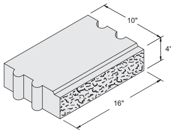
16" x 4" x 10" Dual Lock Item #1061050 84 units / pallet • 50 lbs. / unit
