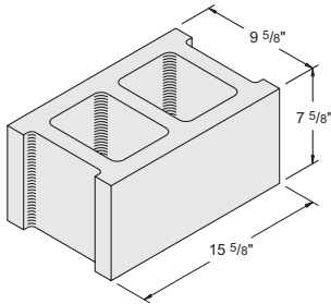
10'' x 8'' x 16'' Hollow Stretcher Item #1020000 87 units / pallet • 44 lbs. / unit
