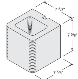
8'' x 8'' x 8'' Half Bullnose Double-End Item #1030375 180 units / pallet • 19 lbs. / unit
