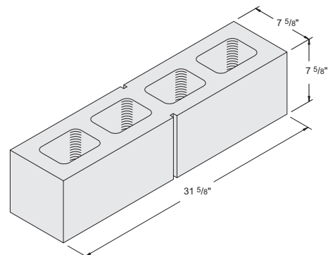
8" x 8" x 32" Double 8 - Light Weight Item #1030940 18 units / pallet • 53.5 lbs. / unit
