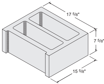
18'' x 8'' x 16'' Hollow Stretcher Item #1061500 36 units / pallet • 70 lbs. / unit
