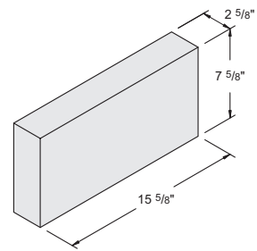
3" x 8" x 16" Solid Item # 1063010 144 units / pallet • 24 lbs. / unit
