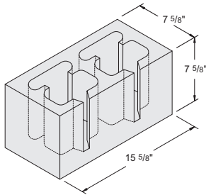
8" x 8" x 16" Soundblox® RCS RF Item #1030330 108 units / pallet • 43 lbs. / unit
