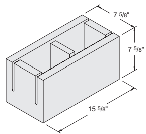
8" x 8" x 16" Bond Beam Knock-Out Item #1030120 108 units / pallet • 42 lbs. / unit
