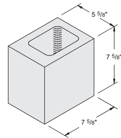
6" x 8" x 8" Half Item #1040030 216 units / pallet • 15 lbs. / unit
