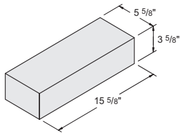
6" x 4" x 16" Solid Item #1050070 168 units / pallet • 25 lbs. / unit
