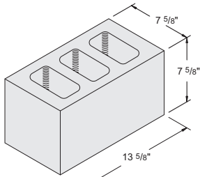
8'' x 8'' x 14'' Item #1030270 105 units / pallet • 40 lbs. / unit ALT: 14'' Half
