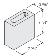
4" x 8" x 8" Half Item # 1050190 360 units / pallet • 13.6 lbs. / unit
