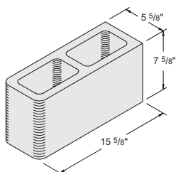
6" x 8" x 16" Bullnose Double-End Item #1040080 132 units / pallet • 33 lbs. / unit
