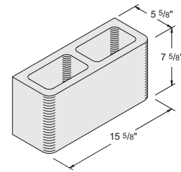
6" x 8" x 16" Bullnose Double-Face Item #1040070 132 units / pallet • 30 lbs. / unit
