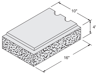
16" x 4" x 10" Dual Lock Left End Item #1061081 44 units / pallet • 48 lbs. / unit
