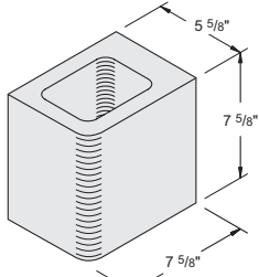
6" x 8" x 8" Half Bullnose Single-Face Item #1040240 216 units / pallet • 15 lbs. / unit
