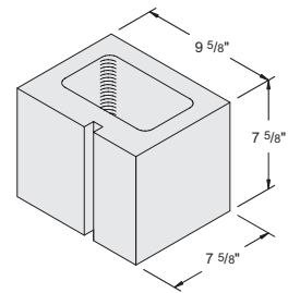
10'' x 8'' x 8'' Half Item #1020040 144 units / pallet • 24 lbs. / unit
