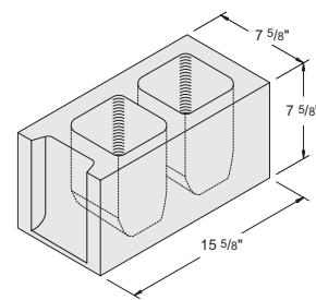
8" x 8" x 16" Termite Item #1030040 72 units / pallet • 49.8 lbs. / unit
