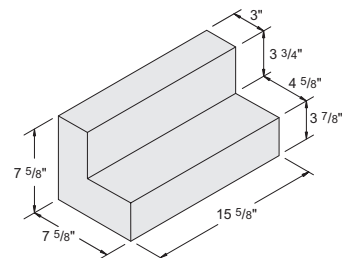
8" x 8" x 16" 4x4 Cut Out Solid Header Item #1030175 72 units / pallet • 53 lbs. / unit
