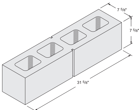
8" x 8" x 32" Double 8 Item #1030950 18 units / pallet • 65 lbs. / unit
