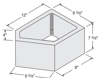
10'' 45° Angle Item #1020020 60 units / pallet • 39 lbs. / unit
