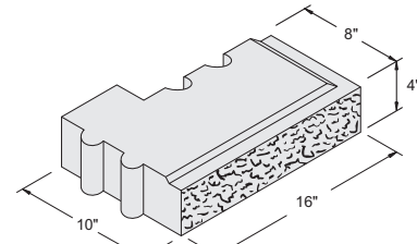
16" x 4" x 10" x 8" Dual Lock Right Corner Item #1061072 44 units / pallet • 45 lbs. / unit
