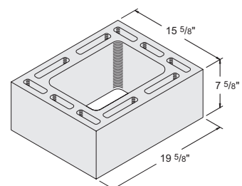
8'' x 12'' Chimney Block Item #1088772 30 units / pallet • 102 lbs. / unit
