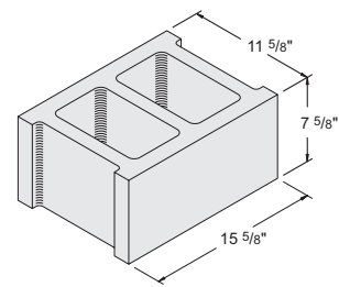
12'' x 8'' x 16'' Hollow Stretcher Item #1010000 78 units / pallet • 48.5 lbs. / unit
