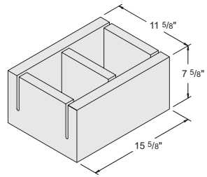
12'' x 8'' x 16'' Bond Beam Knock-Out Item #1010050 72 units / pallet • 55.5 lbs. / unit
