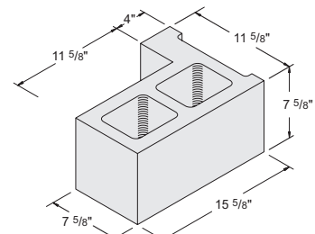
12'' x 8'' x 16'' L Corner Item #1010010 84 units / pallet • 46.6 lbs. / unit
