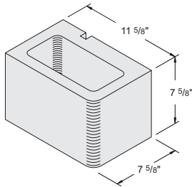
12'' x 8'' x 8'' Half Bullnose Single-Face Item #1010590 144 units / pallet • 30 lbs. / unit
