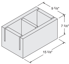
10" x 8" x 16" Bond Beam Knock-Out Item #1020100 72 units / pallet • 47 lbs. / unit
