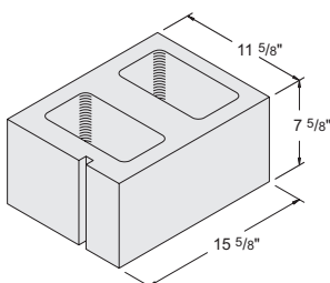
12'' x 8'' x 16'' Jamb Item #1010020 84 units / pallet • 54 lbs. / unit
