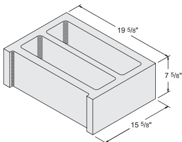
20'' x 8'' x 16'' Hollow Stretcher Item #1061520 36 units / pallet • 89 lbs. / unit
