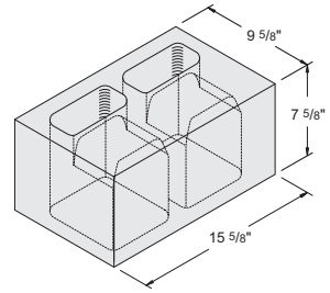
10" x 8" x 16" Brickledge Item #1020051 72 units / pallet • 60 lbs. / unit
