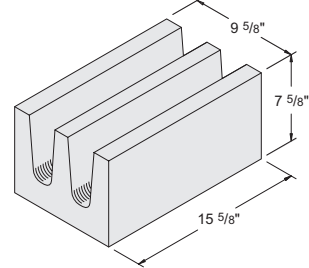
10" x 8" x 16" U-Shaped Lintel Item #1020260 70 units / pallet • 28 lbs. / unit
