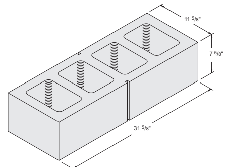
12'' x 8'' x 32'' Double 12 - Light Weight Item #1010930 12 units / pallet • 73.35 lbs. / unit
