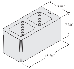
8" x 8" x 16" Bullnose Double-End Item #1030260 108 units / pallet • 34 lbs. / unit
