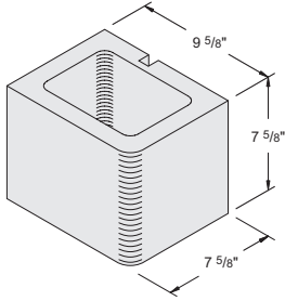
10'' x 8'' x 8'' Half Bullnose Single-Face Item #1020170 144 units / pallet • 23.6 lbs. / unit
