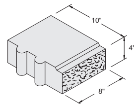
8" x 4" x 10" Dual Lock Right Half Item #1061062 44 units / pallet • 26 lbs. / unit
