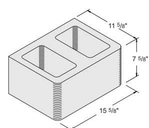
12'' x 8'' x 16'' Bullnose Double-Face Item #1010550 78 units / pallet • 45 lbs. / unit
