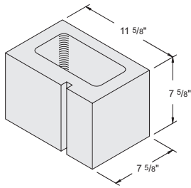
12'' x 8'' x 8'' Half Item #1010030 144 units / pallet • 31 lbs. / unit
