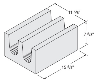
12'' x 8'' x 16'' U-Shaped Lintel Item #1010200 48 units / pallet • 78 lbs. / unit
