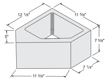
12'' 45° Angle Item #1010140 48 units / pallet • 50 lbs. / unit
