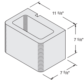
12'' x 8'' x 8'' Half Bullnose Double-End Item #1010600 144 units / pallet • 35 lbs. / unit
