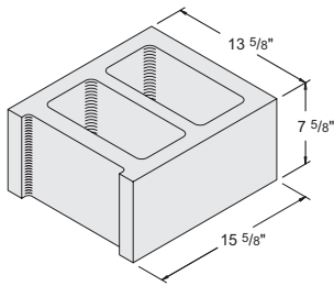
14'' x 8'' x 16'' Hollow Stretcher Item #1060000 54 units / pallet • 59 lbs. / unit
