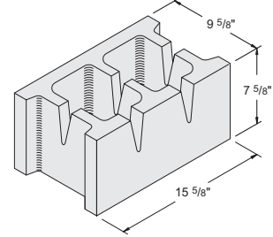
10" x 8" x 16" Drain Item #1020080 87 units / pallet • 43.8 lbs. / unit
