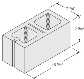
8" x 8" x 16" Jamb Item #1030010 108 units / pallet • 37.5 lbs. / unit
