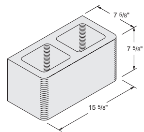
8" x 8" x 16" Bullnose Double-Face Item #1030250 108 units / pallet • 36.3 lbs. / unit
