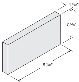
2" x 8" x 16" Solid Item # 1063000 288 units / pallet • 15 lbs. / unit
