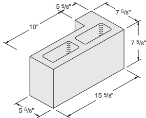
6" x 8" x 16" L Corner Item #1040300 108 units / pallet • 30.2 lbs. / unit
