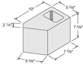
6" 45° Angle Item #1040280 96 units / pallet • 26 lbs. / unit
