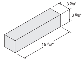
4" x 4" x 16" Solid Item # 1050060 252 units / pallet • 15 lbs. / unit
