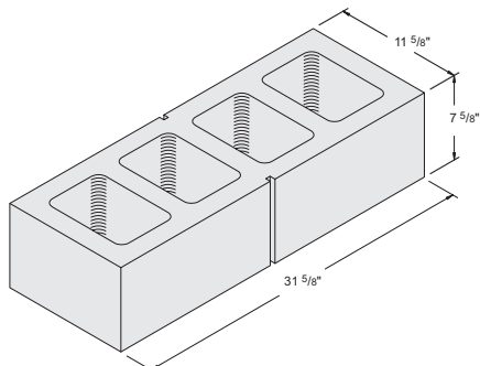
12'' x 8'' x 32'' Double 12 Item #1010920 12 units / pallet • 90.0 lbs. / unit
