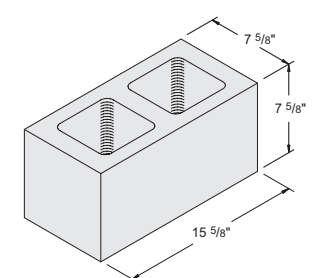
8'' x 8'' x 16'' Pier Item #1030050 108 units / pallet • 36 lbs. / unit
