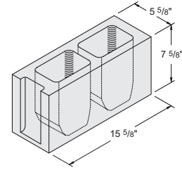
6" x 8" x 16" Termite Item #1040010 108 units / pallet • 35.3 lbs. / unit
