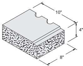
8" x 4" x 10" Dual Lock Left Half Item #1061061 44 units / pallet • 26 lbs. / unit
