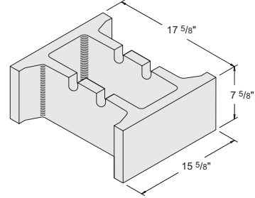
18'' x 8'' x 16'' Grout Item #1061510 54 units / pallet • 70 lbs. / unit
