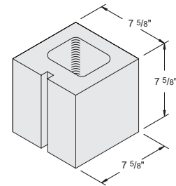
8'' x 8'' x 8'' Half Item #1030020 180 units / pallet • 21 lbs. / unit
