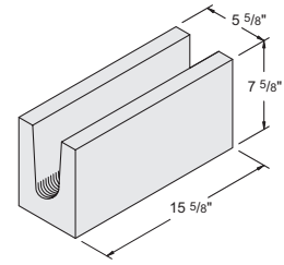
6" x 8" x 16" U-Shaped Lintel Item #1040190 96 units / pallet • 25 lbs. / unit
