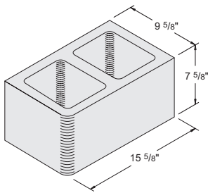
10'' x 8'' x 16'' Bullnose Single-Face Item #1020130 87 units / pallet • 44 lbs. / unit
