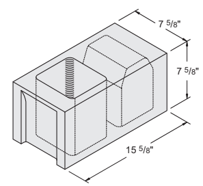
8" x 8" x 16" Anchor Block Item #1030041 90 units / pallet • 42 lbs. / unit
