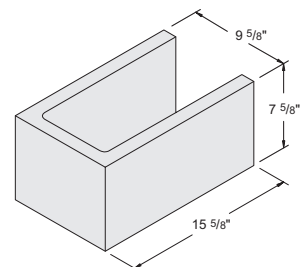
10'' x 8'' x 16'' Beam Lintel (Hairpin) Item #1020280 75 units / pallet • 45 lbs. / unit
