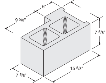
10" x 8" x 16" L Corner Item #1020010 87 units / pallet • 43 lbs. / unit
