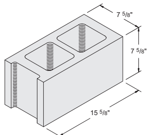
8'' x 8'' x 16'' Hollow Stretcher Item #1030000 108 units / pallet • 36.5 lbs. / unit
