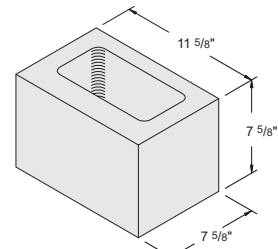
12'' x 8'' x 8'' Half No Slot Item #1010130 144 units / pallet • 32.2 lbs. / unit
