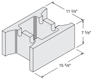
12'' x 8'' x 16'' Grout Item #1010220 72 units / pallet • 46 lbs. / unit
