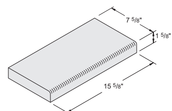
8" x 2" x 16" Curb Item #1063025 216 units / pallet • 12 lbs. / unit
