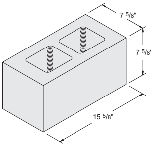
8'' x 8'' x 16'' 57% Solid Item #1030340 108 units / pallet • 40 lbs. / unit
