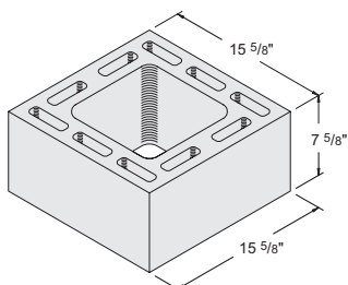
8'' x 8'' Chimney Block Item #1088770 45 units / pallet • 86 lbs. / unit
