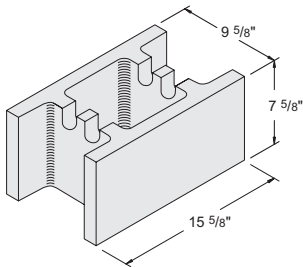
10" x 8" x 16" Grout Item #1020070 84 units / pallet • 43 lbs. / unit
