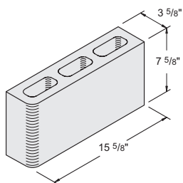
4" x 8" x 16" Bullnose Single-Face Item # 1050400 162 units / pallet • 23 lbs. / unit
