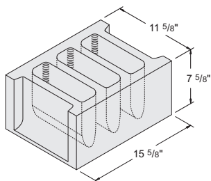
12'' x 8'' x 16'' Termite Item #1010040 54 units / pallet • 70 lbs. / unit
