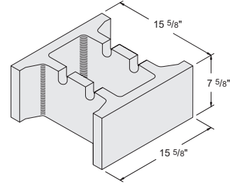
16'' x 8'' x 16'' Grout Item #1061030 54 units / pallet • 54 lbs. / unit
