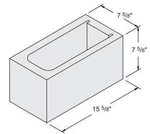
8" x 8" x 16" Beam Lintel (Hairpin) Item #1030390 108 units / pallet • 35 lbs. / unit
