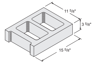
12'' x 4'' x 16'' Half High Item #1010180 120 units / pallet • 28 lbs. / unit MIXED: Jamb 1:1 Ratio
