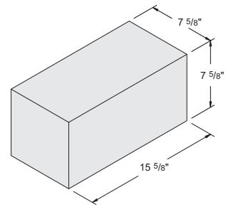
8'' x 8'' x 16'' Solid Item #1030140 54 units / pallet • 68.5 lbs. / unit
