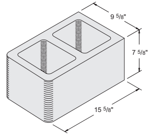
10'' x 8'' x 16'' Bullnose Double-End Item #1020190 87 units / pallet • 43 lbs. / unit
