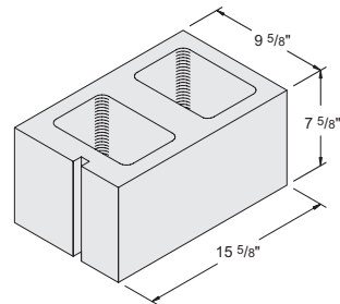
10'' x 8'' x 16'' Jamb Item #1020030 87 units / pallet • 44 lbs. / unit
