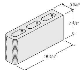
4" x 8" x 16" Bullnose Double-End Item # 1050410 162 units / pallet • 25 lbs. / unit
