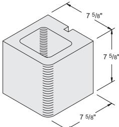
8'' x 8'' x 8'' Half Bullnose Single-Face Item #1030280 180 units / pallet • 21 lbs. / unit
