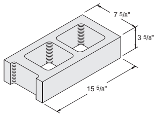
8'' x 4'' x 16'' Half High Item #1070460 162 units / pallet • 17 lbs. / unit MIXED WITH: Splittable Jambs, Grout Block, & Stretchers
