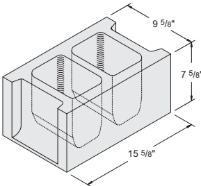
10" x 8" x 16" Termite Item #1020050 54 units / pallet • 59 lbs. / unit
