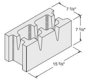
8" x 8" x 16" Drain Item #1030002 90 units / pallet • 35 lbs. / unit
