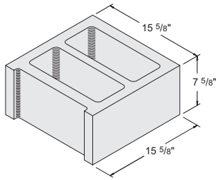
16'' x 8'' x 16'' Hollow Stretcher Item #1061000 54 units / pallet • 65 lbs. / unit
