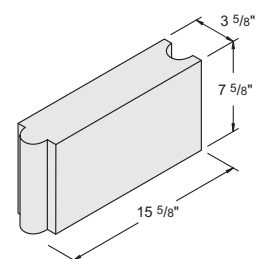
4" x 8" x 16" Mine Block Item # 1050087 108 units / pallet • 31.5 lbs. / unit
