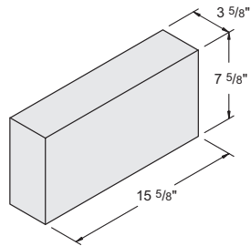
4" x 8" x 16" Solid Item # 1050080 108 units / pallet • 33.2 lbs. / unit
