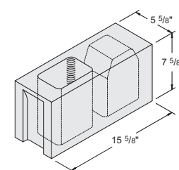
6" x 8" x 16" Anchor Block Item #1040002 120 units / pallet • 31.6 lbs. / unit
