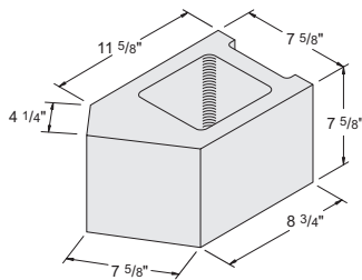
8" 45° Angle Item #1030130 120 units / pallet • 33 lbs. / unit
