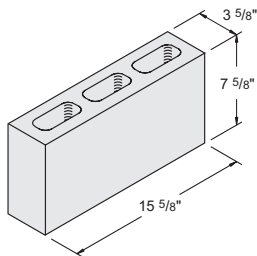
4" x 8" x 16" Hollow Item # 1050000 162 units / pallet • 24 lbs. / unit
