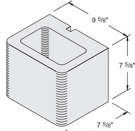
10'' x 8'' x 8'' Half Bullnose Double-End Item #1020180 144 units / pallet • 24 lbs. / unit
