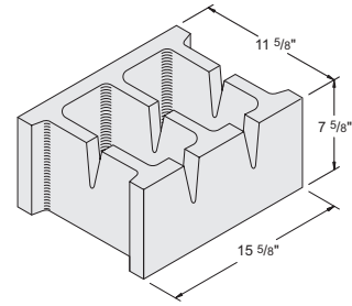
12'' x 8'' x 16'' Drain Item #1010012 66 units / pallet • 40 lbs. / unit
