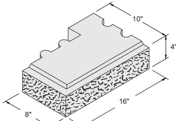
16" x 4" x 10" x 8" Dual Lock Left Corner Item #1061071 44 units / pallet • 45 lbs. / unit
