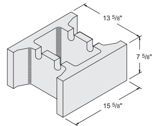
14'' x 8'' x 16'' Grout Item #1060010 54 units / pallet • 58 lbs. / unit
