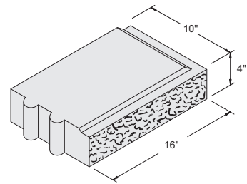
16" x 4" x 10" Dual Lock Right End Item #1061082 44 units / pallet • 48 lbs. / unit
