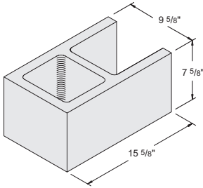
10" x 8" x 16" Conduit Item #1020270 75 units / pallet • 45 lbs. / unit
