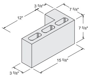
4" x 8" x 16" L Corner Item # 1050160 120 units / pallet • 35 lbs. / unit
