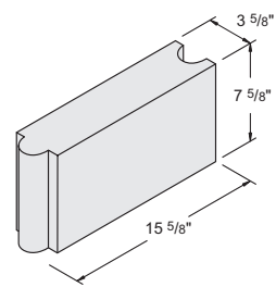
4" x 8" x 16" Mine Block #1050087
