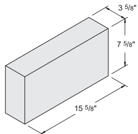
4" x 8" x 16" Solid #1050080
