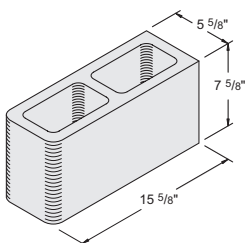
6" x 8" x 16" Bullnose Double-End #1040080
