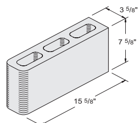
4" x 8" x 16" Bullnose Double-End #1050410
