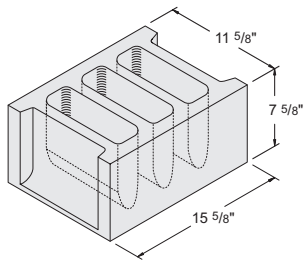
12" x 8" x 16" Termite #1010040
