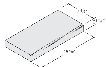
8" x 2" x 16" Curb #1063025
