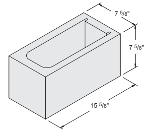
8" x 8" x 16" Beam Lintel (Hairpin) #1030390
