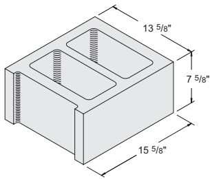
14" x 8" x 16" Hollow Stretcher #1060000
