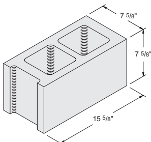
8" x 8" x 16" Hollow Stretcher #1030000
