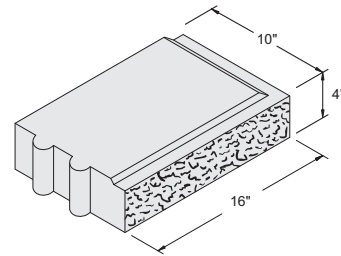
16" x 4" x 10" Dual Lock Right End #1061082
