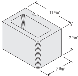
12" x 8" x 8" Half Bullnose Single-Face #1010590
