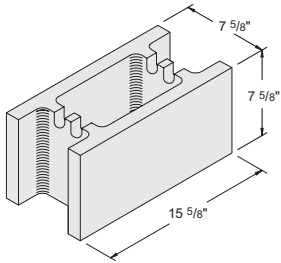
8" x 8" x 16" Grout #1030230
