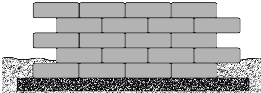
Running Bond Pattern: 3 block per face foot Each 20" x 48" section uses 20 blocks
