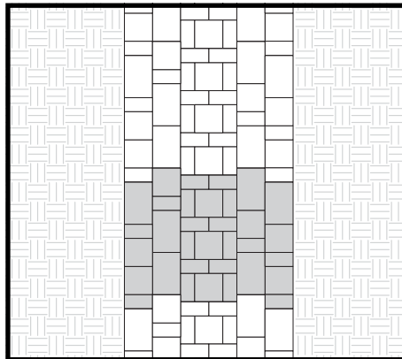
LINEAR WALKWAY PATTERN
