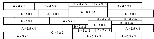
5' x 18' WALL - 90 sq. ft. (Uses 2 A Pallets, 2 B Pallets, & 1 C Pallet)
