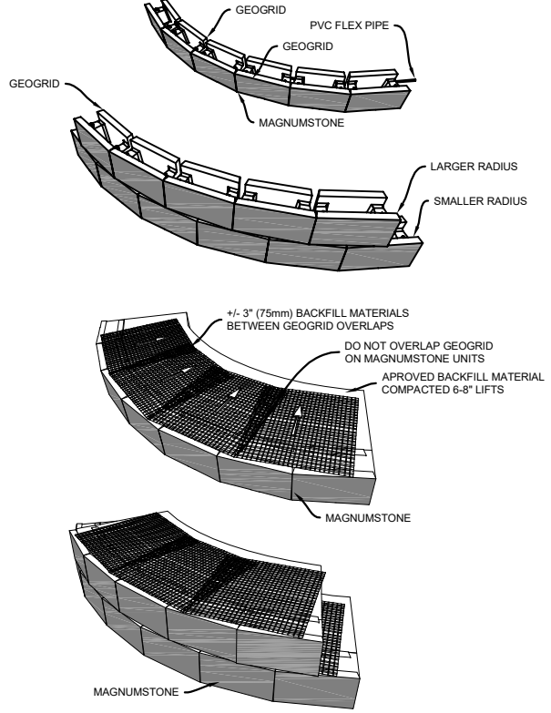
OUTSIDE CURVE
