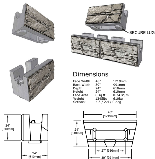
STANDARD UNIT
