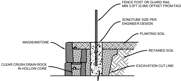
RAILING BEHIND WALL
