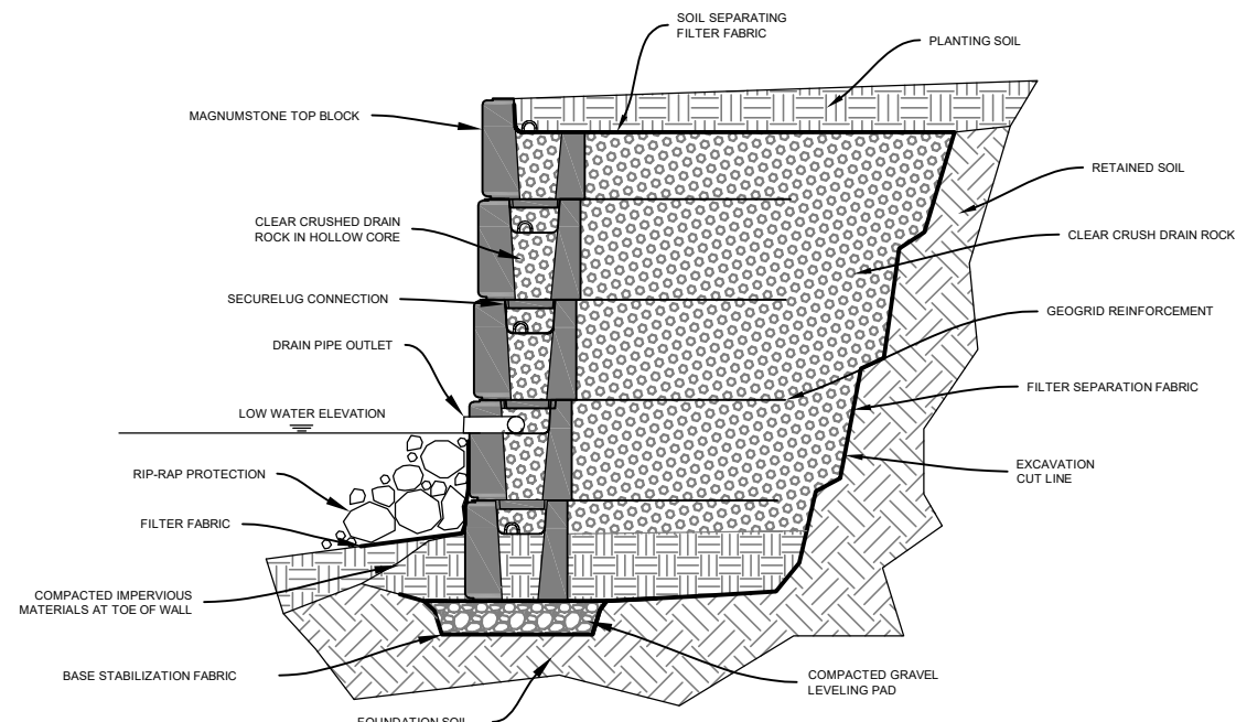
WATER APPLICATION
