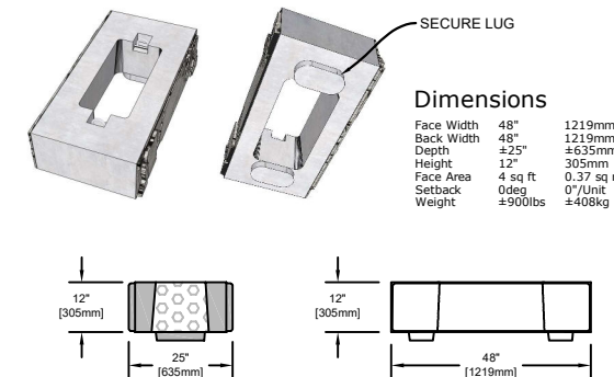
DOUBLE SIDED FREESTANDING UNIT
