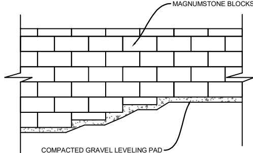
BASE STEP UP
