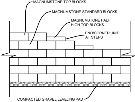
TOP OF WALL STEP UP
