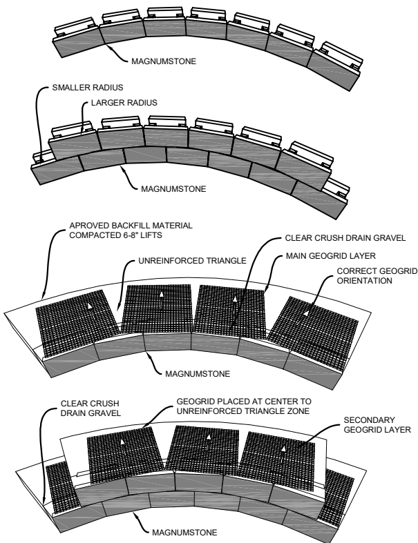
INSIDE CURVE
