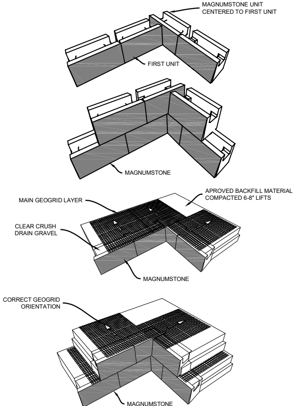
INSIDE CORNER
