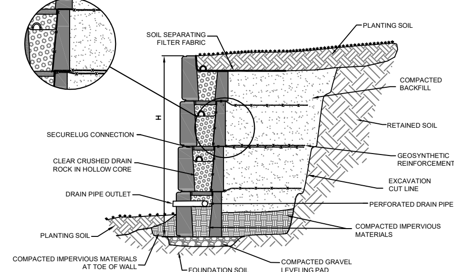
POSITIVE CONNECTION REINFORCED WALL
