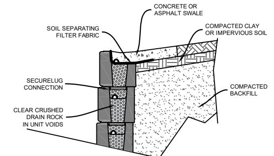
CONCRETE / ASPHALT SWALE
