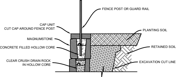
RAILING THROUGH HOLLOW CORE W /CAP
