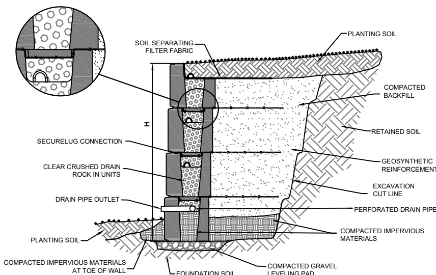
GEOGRID REINFORCED WALL
