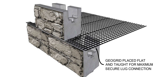
GEOGRID REINFORCEMENT
