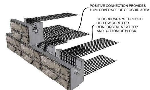
POSITIVE CONNECTION
