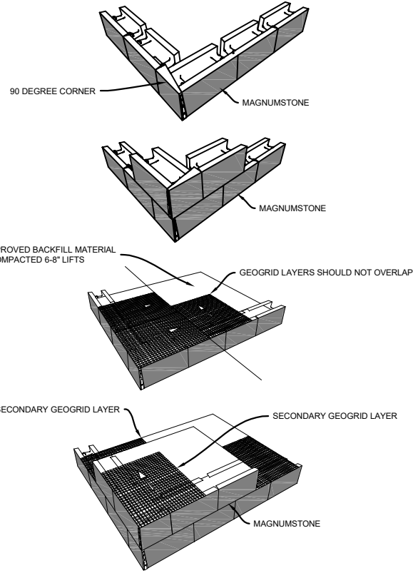
OUTSIDE CORNER
