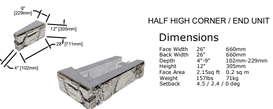
CORNER/END UNIT
