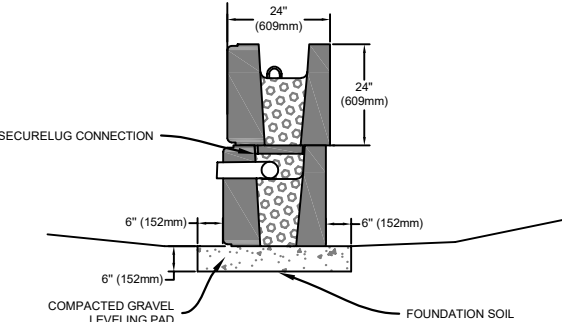
LEVELING PAD
