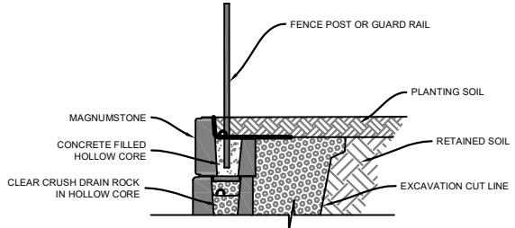
RAILING THROUGH HOLLOW CORE
