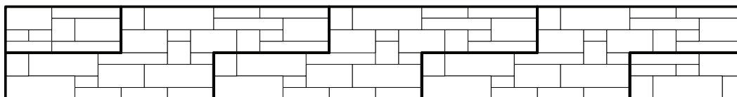
24" High Wall: 24" x 16' Wall Section Shown = 32 face sq. ft. (1 1/2 Wall Pallet)
